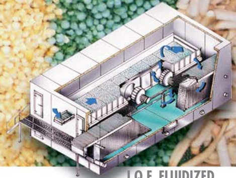
I.Q.F. FLUIDIZED TRAY FREEZER
