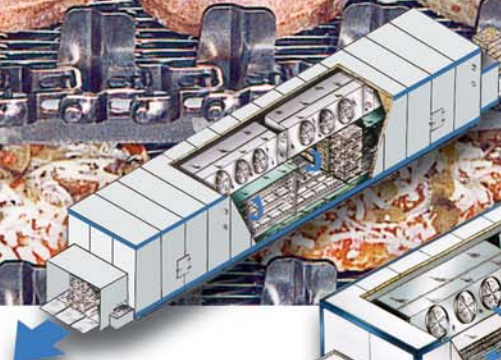
DRAG-THRU DOLLY TUNNEL FREEZER POULTRY, MEATS & SEAFOOD OR PACKAGED BOX PRODUCTS
