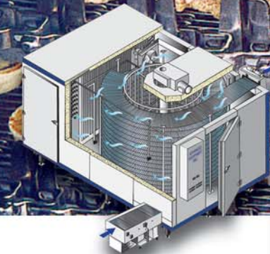
I.Q.F. PACKAGED SPIRAL FREEZER
